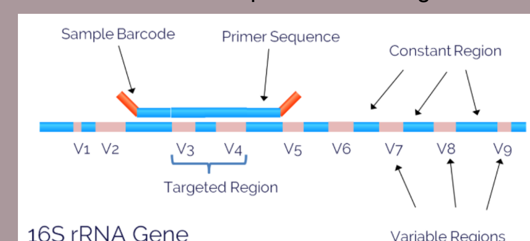
Figure 1. Barcoded Primer Sequence Attaching to a 16S rRNA Gene
