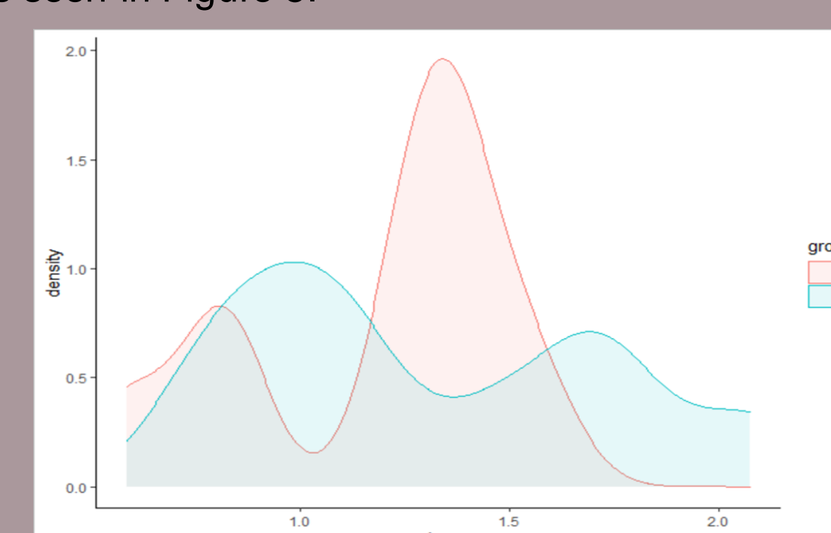
Figure 5. Distribution of Shannon Diversity Scores of the FM and Control Groups (Mann-Whitney U = 38 , p = 0.596 ).
