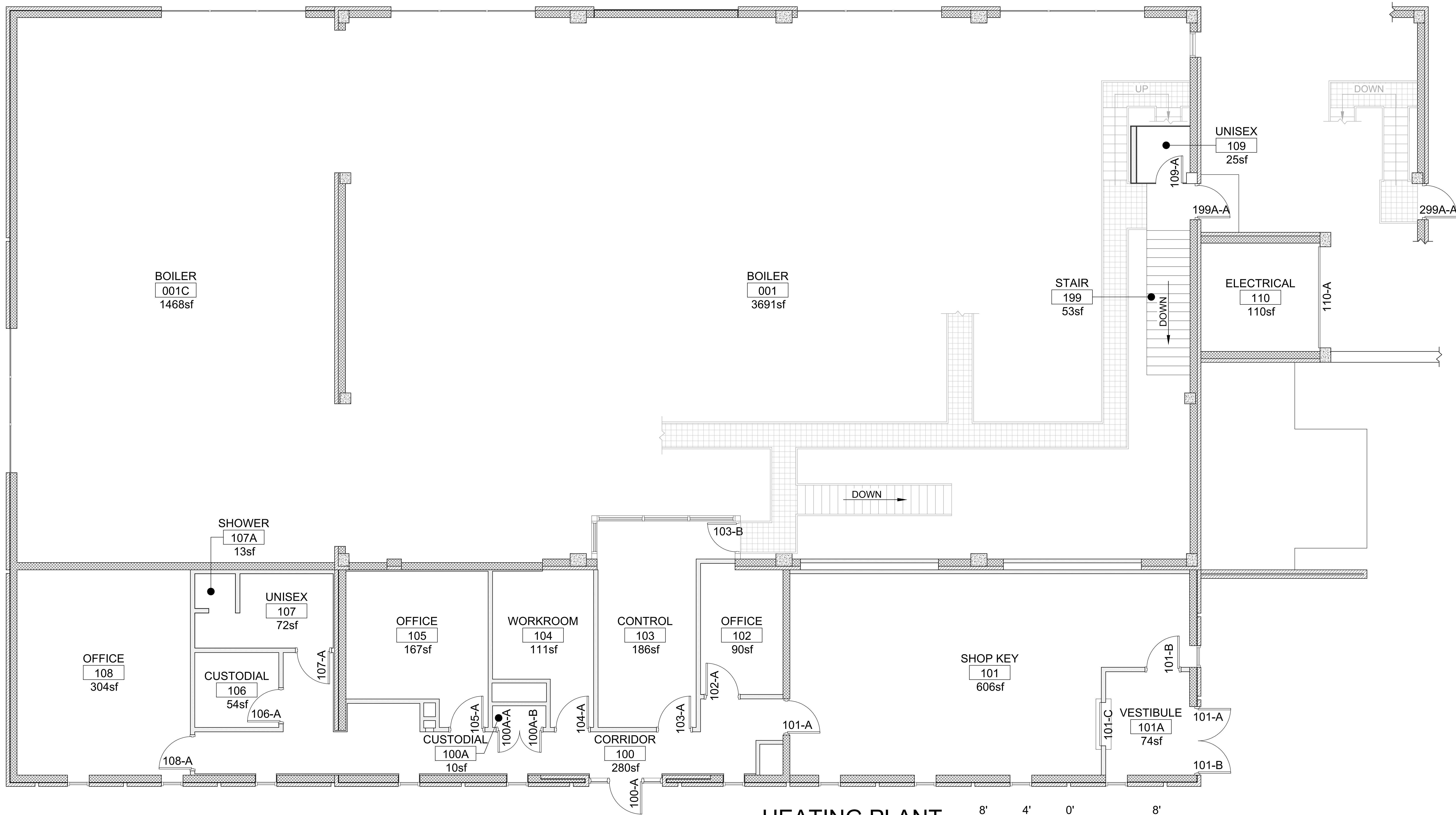
HEATING PLANT FIRST FLOOR PLAN
