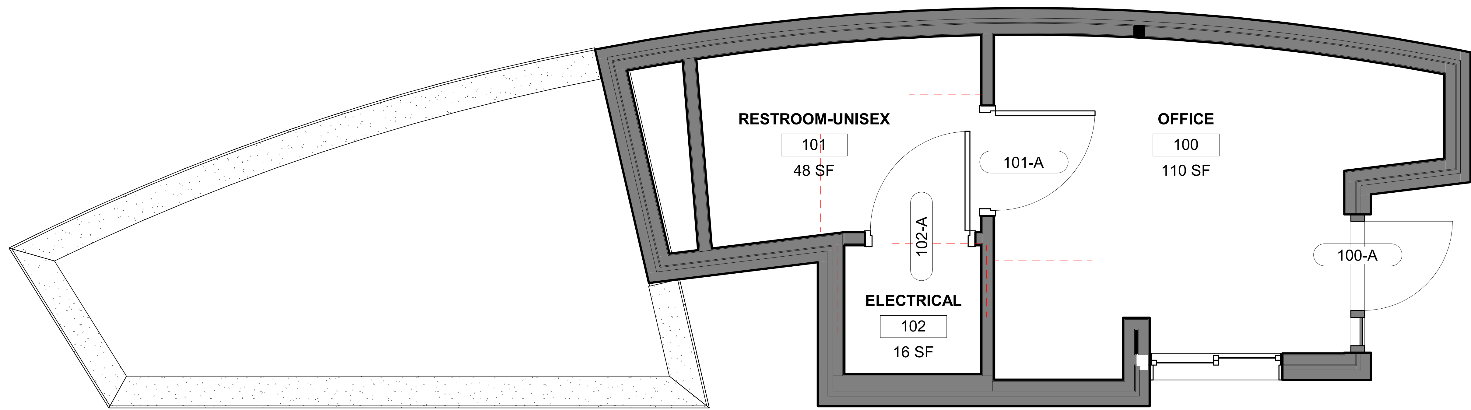
1 IN Floor Plan 3/8" = 1'-0"
