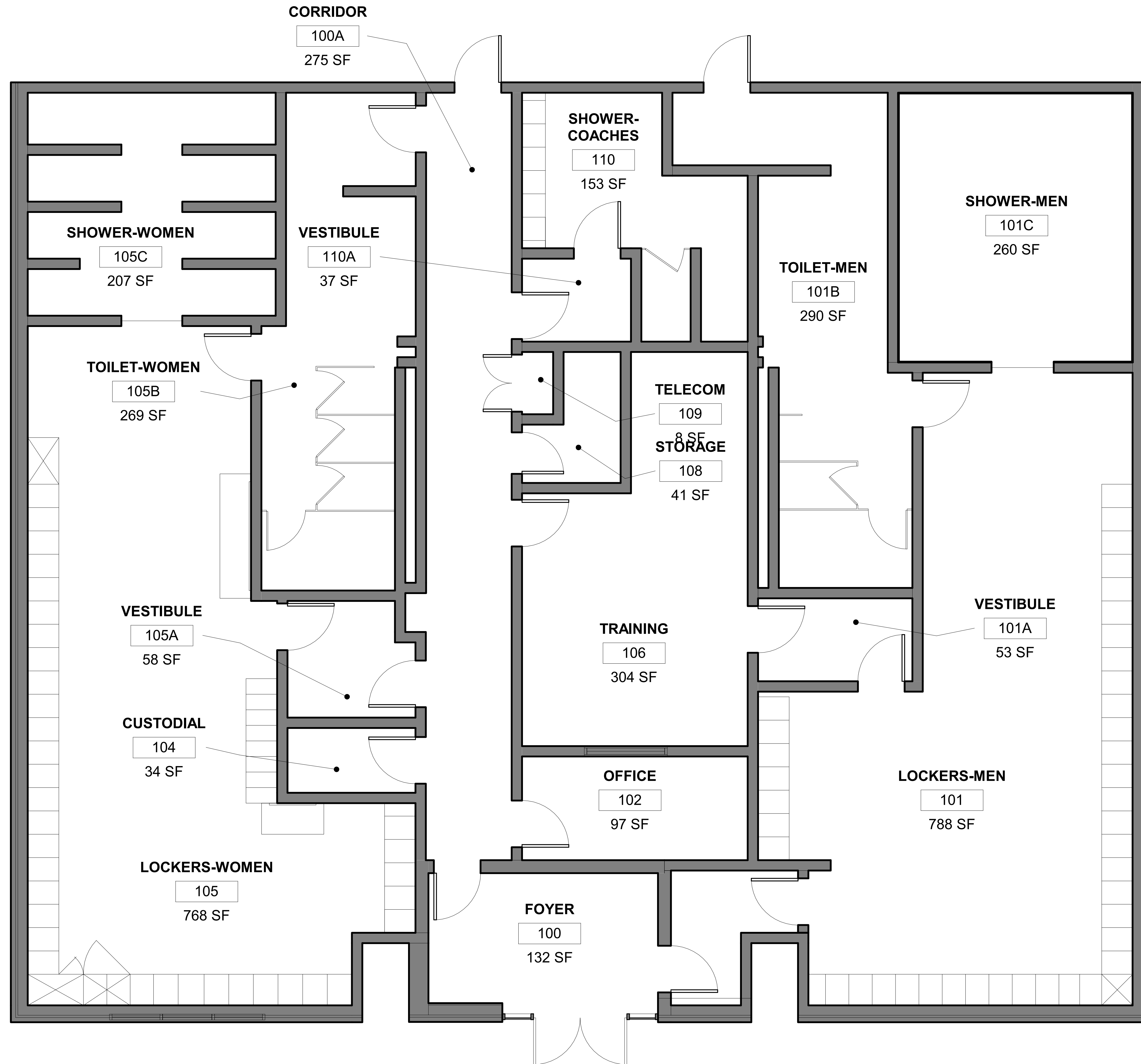
① TR Level 1 Access Plan 3/16" = 1'-0"
